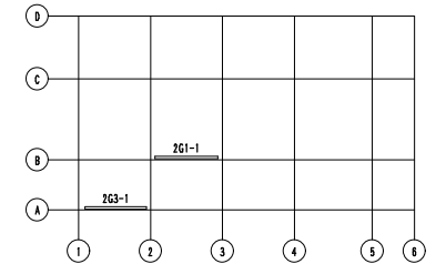
2 KEY PLAN
